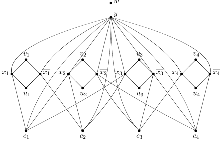
Figure 3. A construction of G(I) for (x_1 \vee x_2 \vee x_3) \wedge (\bar{x}_1 \vee x_2 \vee x_3) \wedge (\bar{x}_2 \vee \bar{x}_3 \vee x_4) \wedge (\bar{x}_2 \vee \bar{x}_3 \vee \bar{x}_4) .
