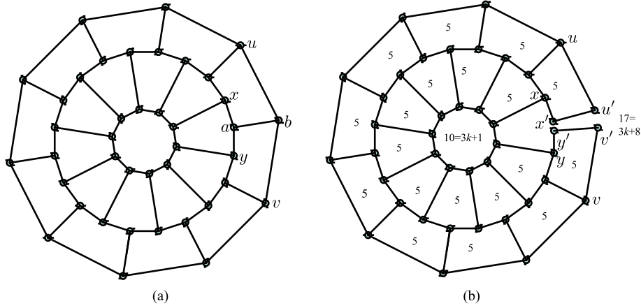
Figure 4. The graph GP(6k + 2, 2) for k = 3 .
