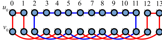
Figure 7. Another two spanning cycles for GP(3k+2, 3) for k=4 .
