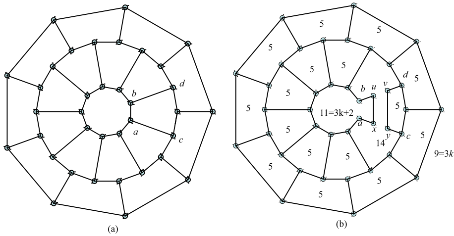
Figure 3. The graph GP(6k, 2) for k = 3 .
