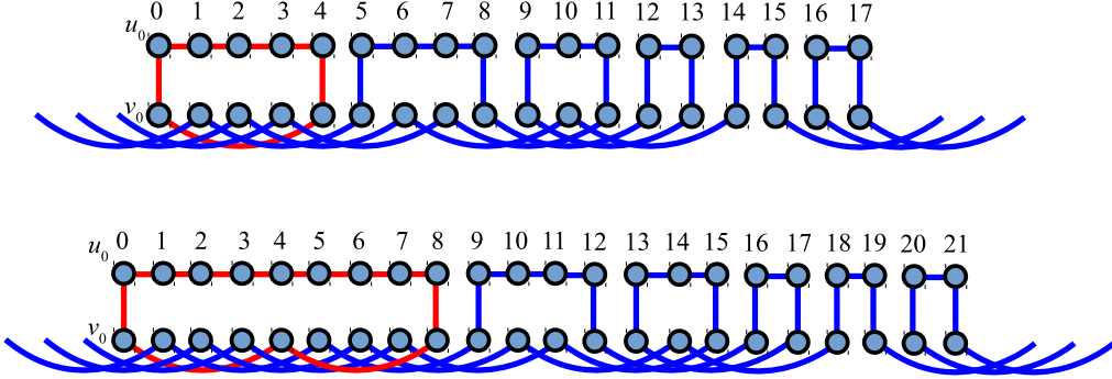
Figure 14. Two spanning cycles for GP(4r + 2, 4) for r = 4, 5 .
