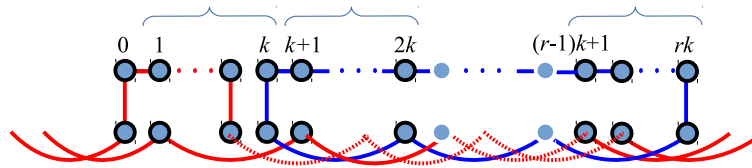
Figure 1. The two spanning cycles of GP(rk + 1, k) .
