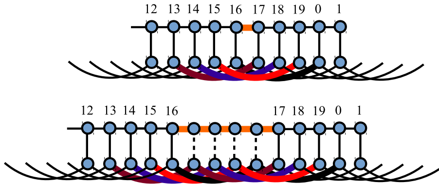
Figure 11. Expanding the graph from GP(20, 4) to GP(24, 4) .
