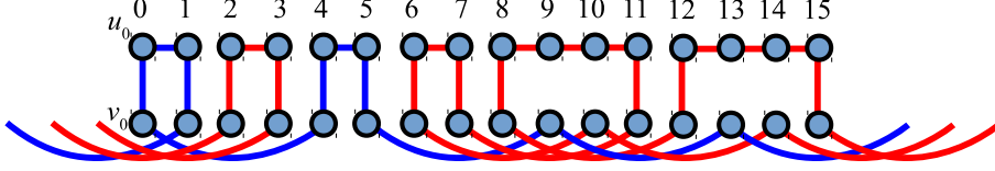
Figure 13. Two spanning cycles for GP(4r, 4) for r = 4 .
