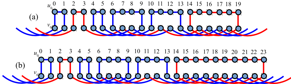
Figure 10. Another two spanning cycles for GP(4r, 4) for r = 5 and r = 6 .
