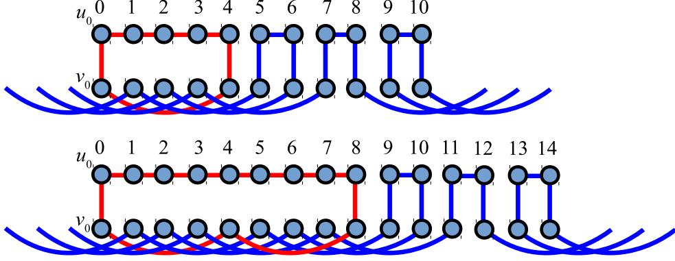
Figure 16. Two spanning cycles for GP(4r + 3, 4) for r = 2, 3 .
