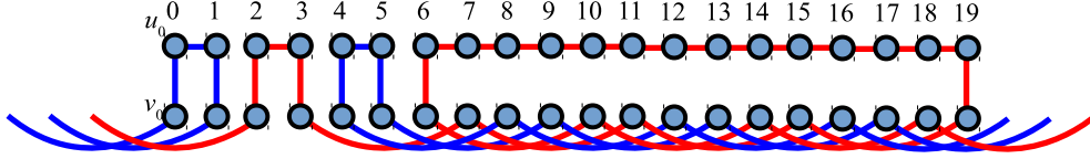
Figure 9. Two spanning cycles for GP(4r, 4) for r = 5 .
