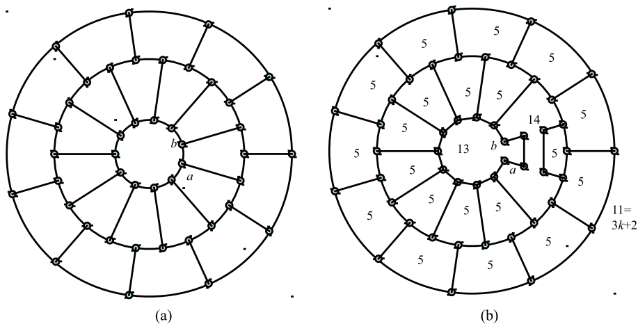
Figure 5. The graph GP(6k + 4, 2) for k = 3 .
