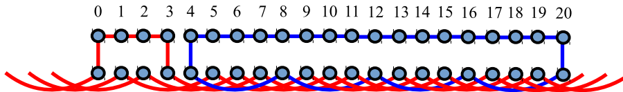
Figure 2. The two spanning cycles of GP(21, 4) .
