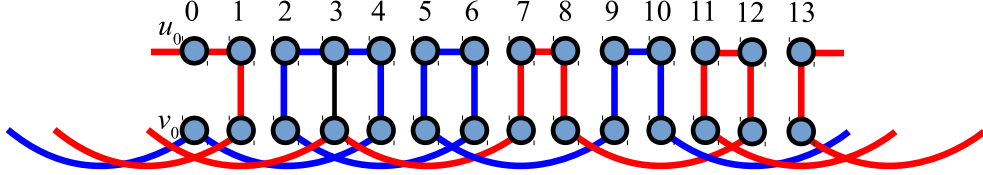
Figure 15. Two spanning cycles for GP(4r + 2, 4) for r = 3 .
