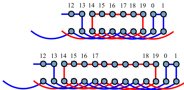
Figure 12. Expanding a pair of valid cycles from GP(20, 4) to GP(24, 4) .
