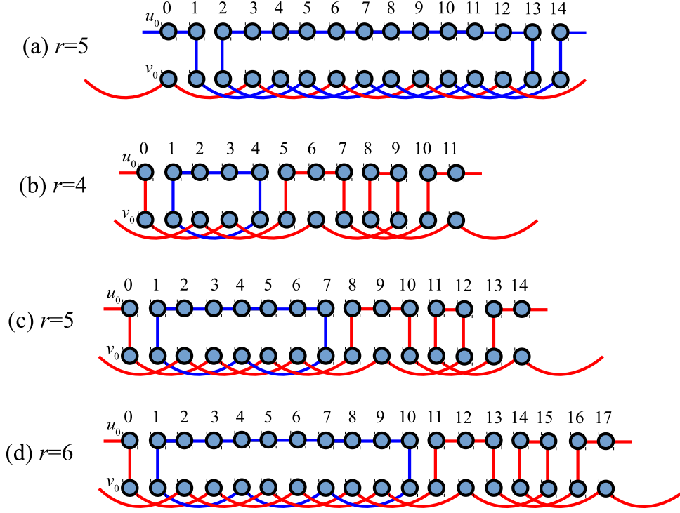
Figure 8. Two spanning cycles for GP(3r, 3) for r = 4, 5, 6 .
