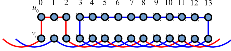
Figure 6. Two spanning cycles for GP(3k+2, 3) for k=4 .
