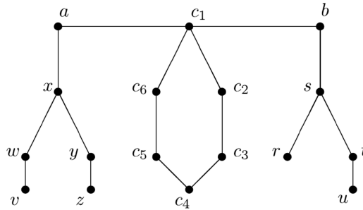
Figure 1. The graph G .
