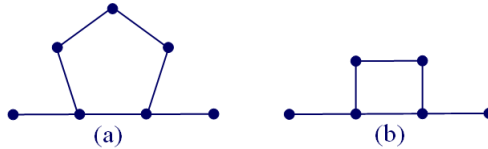
Figure 1. (a) Geodetic graph G . (b) Non-geodetic graph H .
