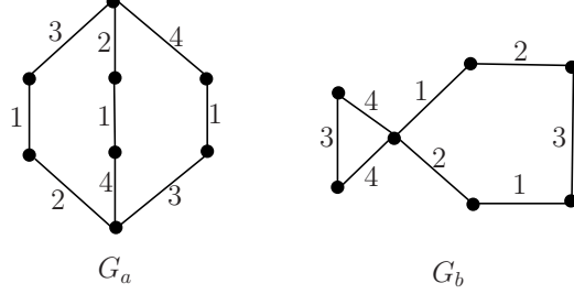
Figure 1. Graphs for Theorem 12 and Corollary 13.
