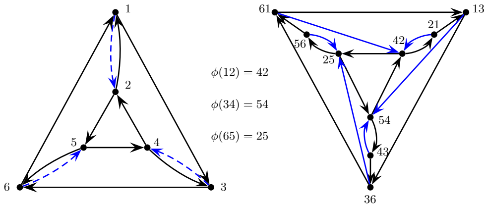
Figure 1. A digraph and its partial line digraph.
