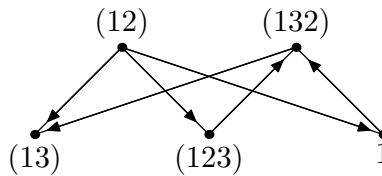
Figure 5. An S_3 -cordial labeling of an orientation of K_{2,3} , with the convention that \sigma\tau means apply \sigma then \tau .
