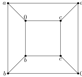
Figure 3. A V_4 -cordial labeling of the cube Q_3 .
