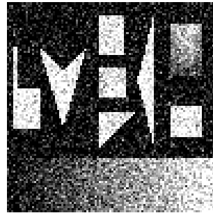
Figure 6. Noisy Image
