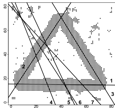
Figure 3. Regression Lines
