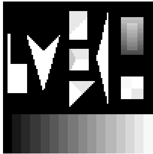
Figure 5. Original Image
